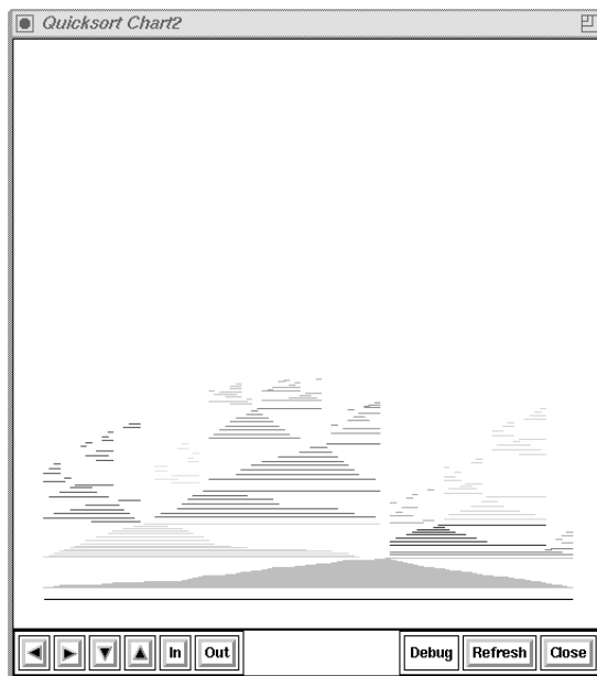
Figure 10: A snapshot of the swap history view of the parallel quicksort program under the serialized ordering.
