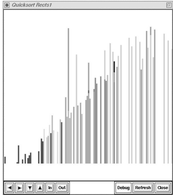
Figure 4: A snapshot of the array view of the parallel quicksort program under the timestamp ordering.
