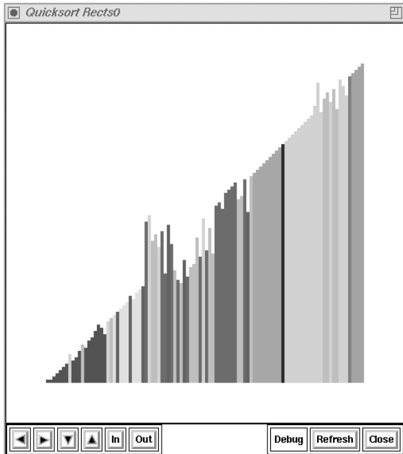
Figure 3: A snapshot of the array view of the parallel quicksort program under a correct ordering.
