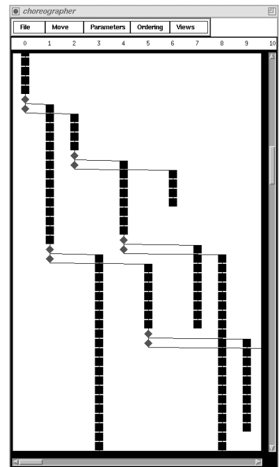
Figure 8: A portion of the execution graph produced by the choreographer. The events are from a parallel quicksort program. The ordering type is maximum concurrency.
