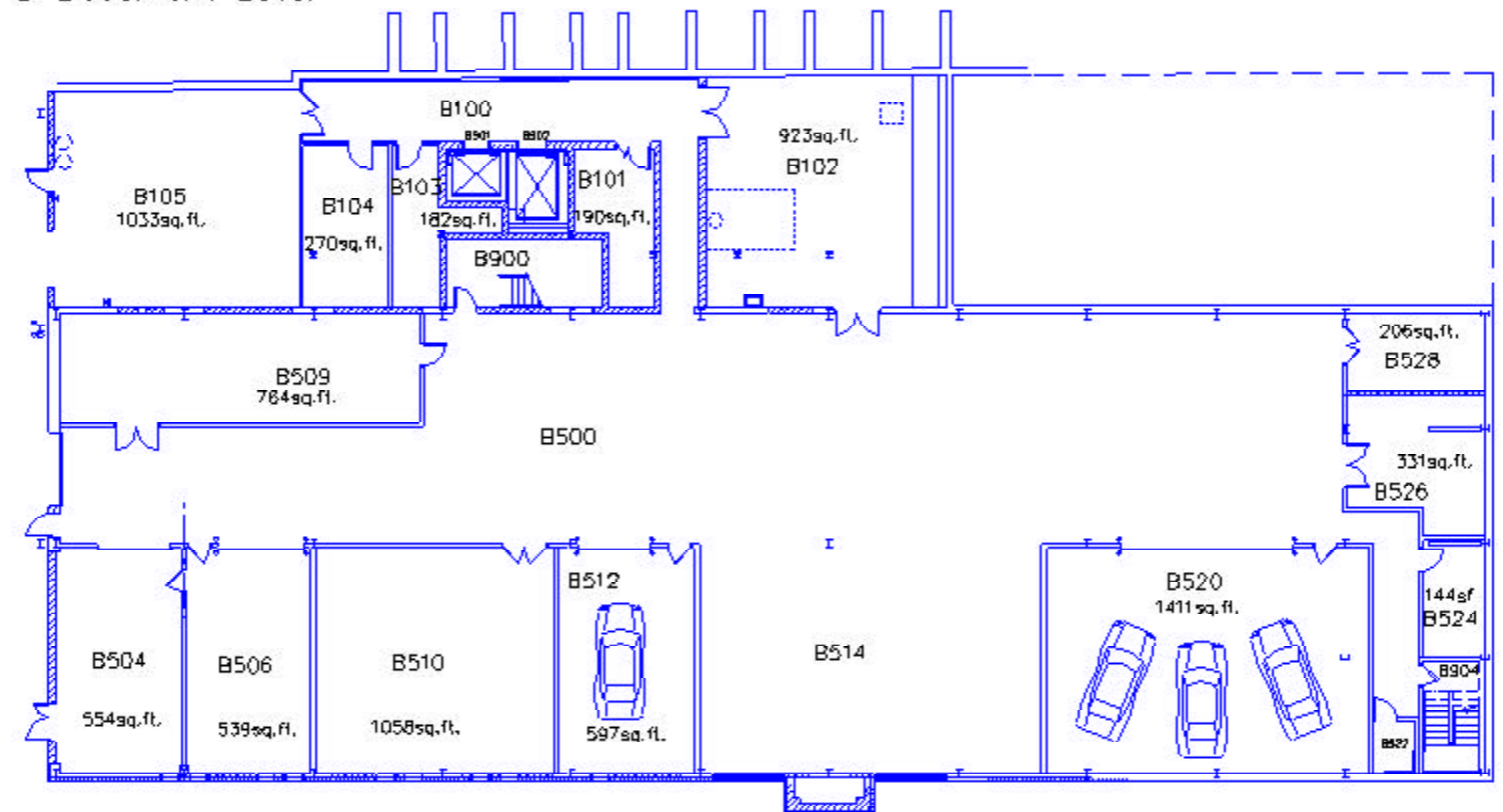
Newell-Simon Hall B Basement Level
