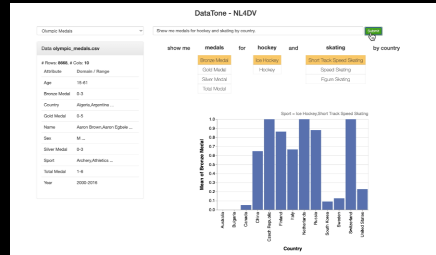
Example 2/4: "Ambiguity Widgets" of DataTone
