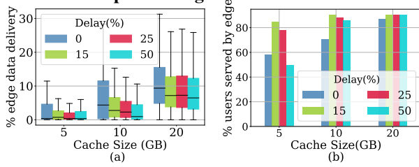
Figure 17: (a) Data delivery to users with 10 edge nodes to users under per node cache sizes (b) Users who got data from edge under various cache and delay parameters.
