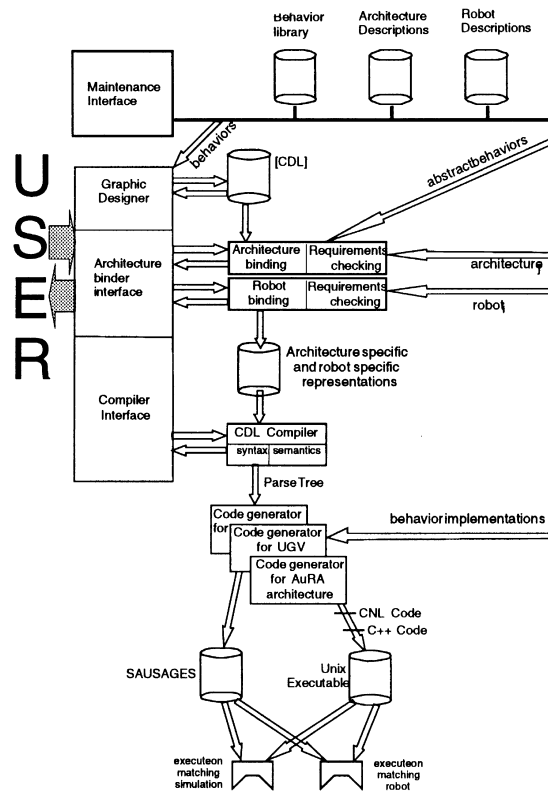
Fig. 4. MissionLab system architecture.
