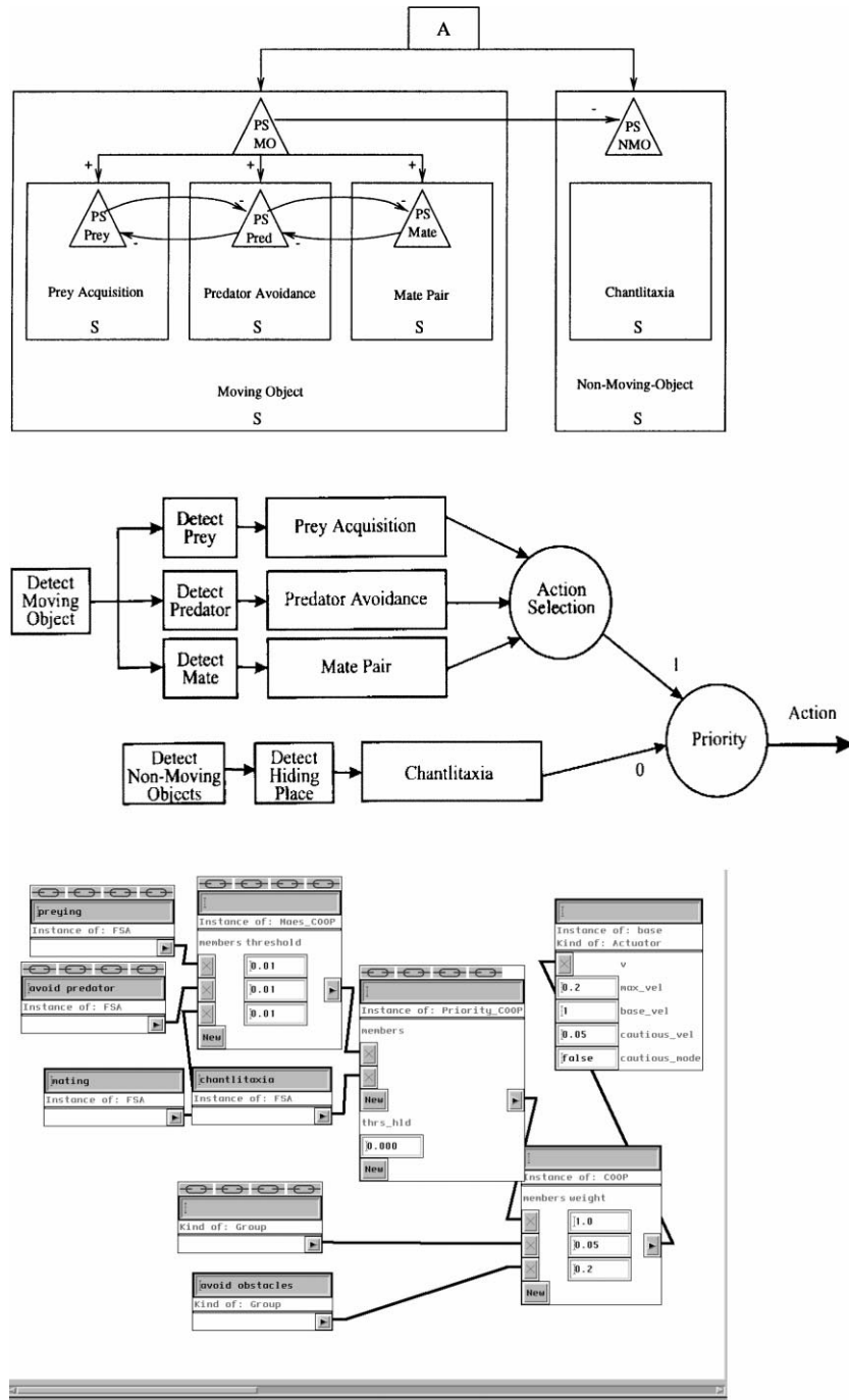
Fig. 7. Visuomotor behaviors of mantis. (Top) Model developed by Cervantes-Pérez. (Middle) Abstract adapted model. (Bottom) Model as implemented in MissionLab .
