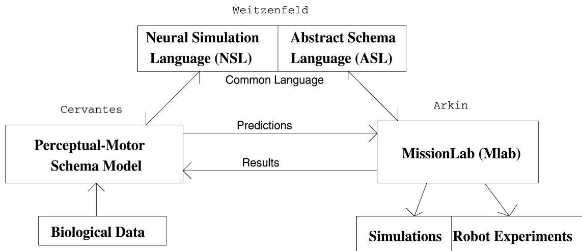
Fig. 3. Schema-based modeling tools connecting neuroscientific studies with robotic control systems.
